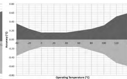
Supplied 'Type A' High Accuracy Thermistor Probe Part Number: EL-PROBEA-3.0M-TP+
